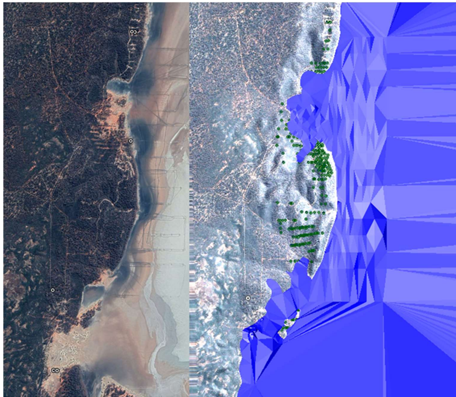
Figure 14-72 Satellite image of the Selene/North Scotia area, with (right) and without (left) the transported material interpretation
