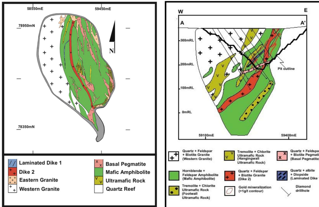
Figure 7-4 Simplified Geology of the Chalice Pit (left) Plan View, (right) Section view looking north Source: Karora
