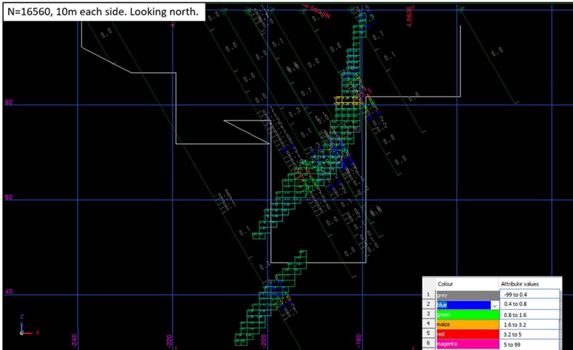
Figure 14-93 Section view of model, drill holes and US$1,600 RPEEE shell at Abbotshall
