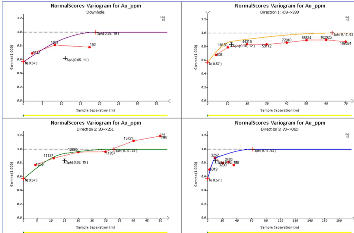
Figure 14-16 Fairplay North variogram – oxide Domains 1 to 3 combined
