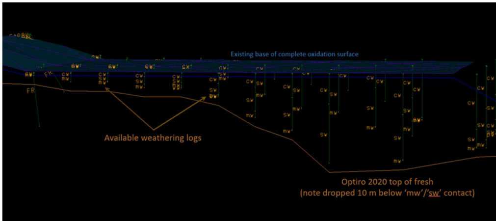
Figure 14-71 Oblique view, looking NNW, showing local modifications to the weathering surface in the Selene/North Scotia area
