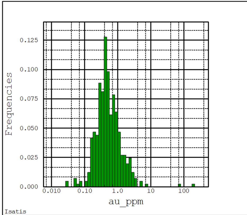
Figure 14-46 Log histogram of uncut gold grade - Domain 100
