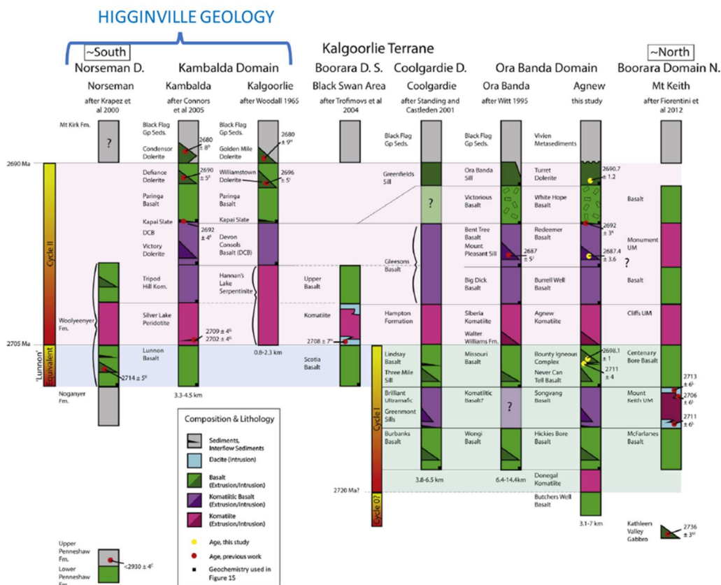
Figure 7-2 Stratigraphic relationships of the principal mafic-ultramafic units of the Kalgoorlie Terrane Source: Hayman (2015)
