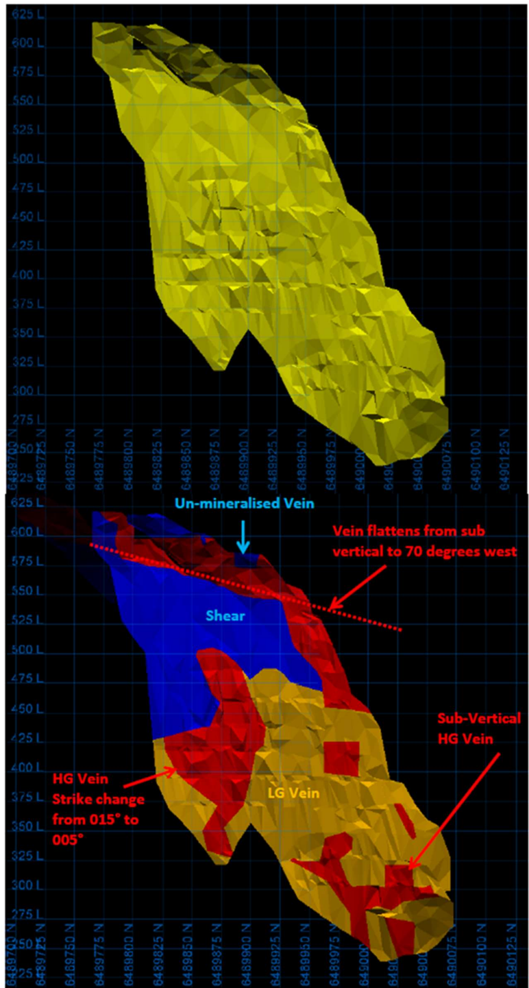
Figure 14-6 Artemis main wireframe (top) and sub-domaining (bottom) – long-section view looking west
