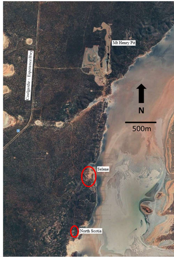
Figure 16-19 Mt Henry Group current layout
