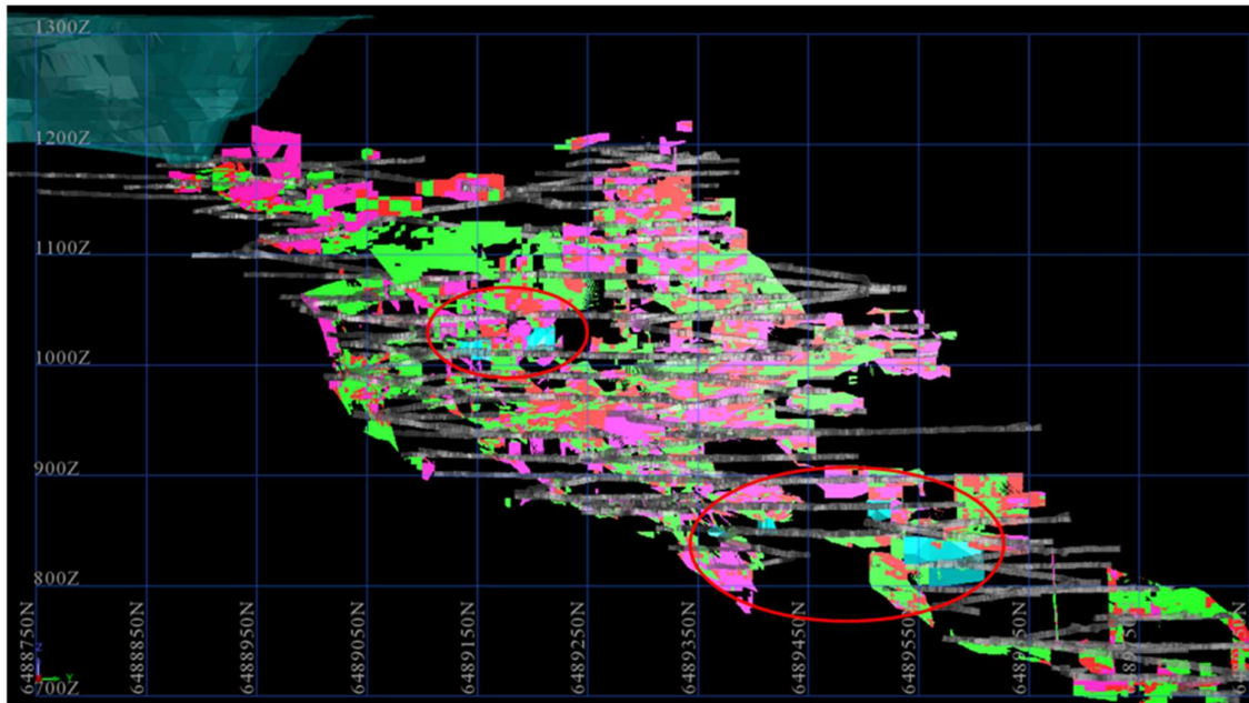
Figure 14-9 Karora sterilisation shapes shown in cyan colour – longsection looking west.
