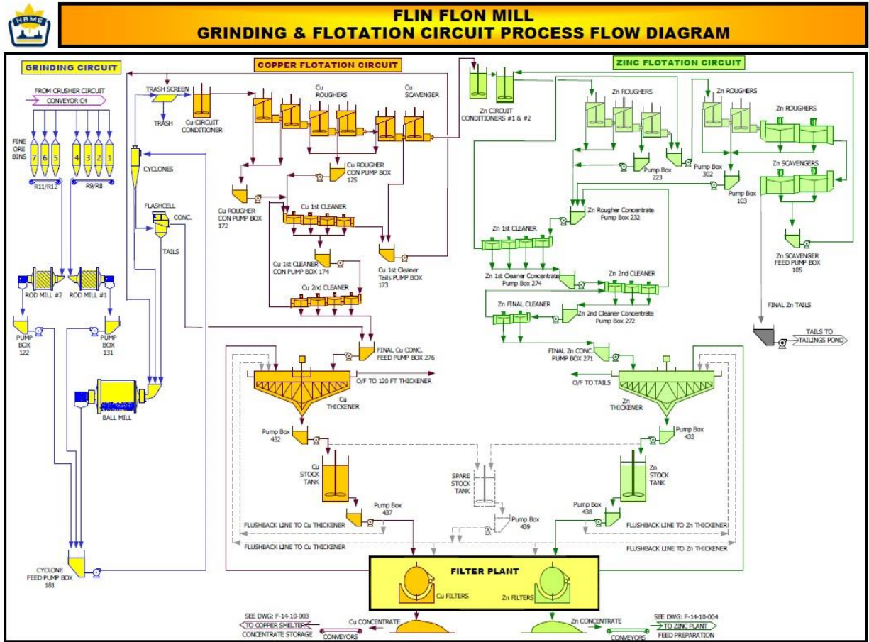
Figure 2: Flin Flon Concentrator Worksheet
